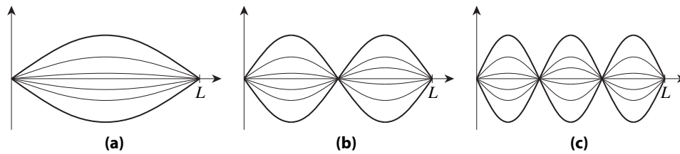
Figure 53.2: The (a) first harmonic, (b) second harmonic, and (c) third harmonic for a vibrating string of length L sketched at various times as functions of x .
