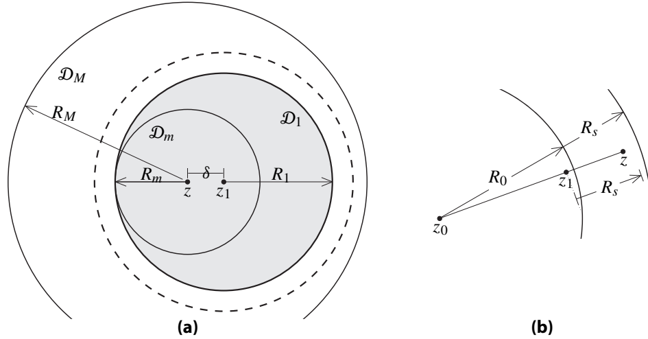
Figure 32.1: (a) Limits on the radius of analyticity at z based on the radius of analyticity R_1 at z_1 , with R_M = R_1 + 2\delta and R_m = R_1 - \delta , and (b) three points in a line with |z - z_0| < R_0 + R_s , |z_1 - z_0| < R_0 and |z - z_1| < R_s .
