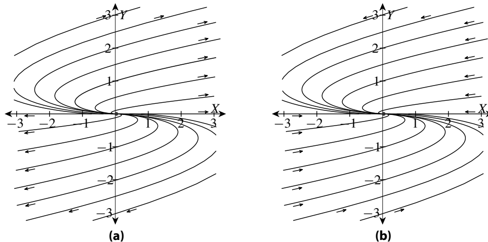
Figure 40.4: Trajectories for a 2 \times 2 system \mathbf{x}' = \mathbf{A}\mathbf{x} when all the eigenvectors of \mathbf{A} are parallel to the X -axis assuming (a) the eigenvalue is positive, and (b) the eigenvalue is negative.
