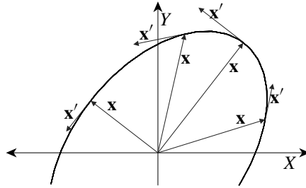
Figure 40.6: The \mathbf{x} and \mathbf{x}' vectors for various points on an elliptic trajectory.
