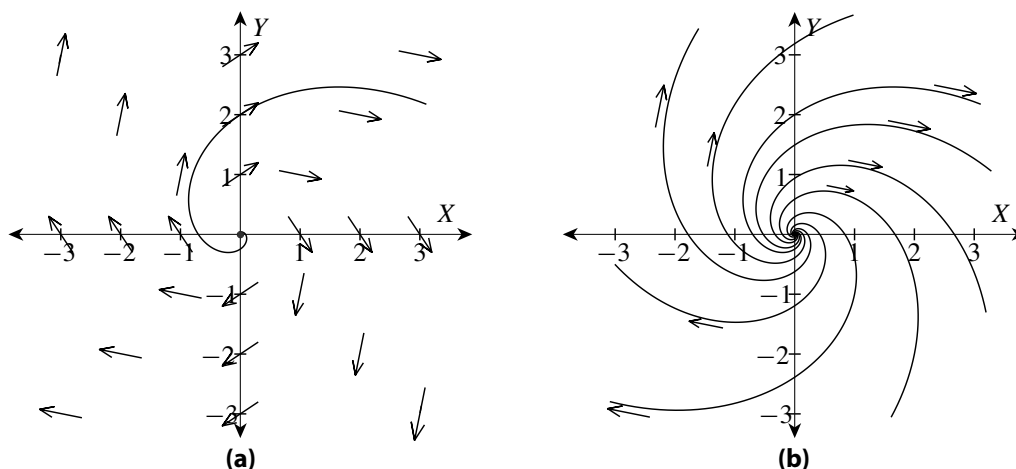
Figure 40.2: (a) A minimal direction field with one ‘matching’ spiral trajectory, and (b) a phase portrait of the system in example 40.3 in which \lambda > 0 .
