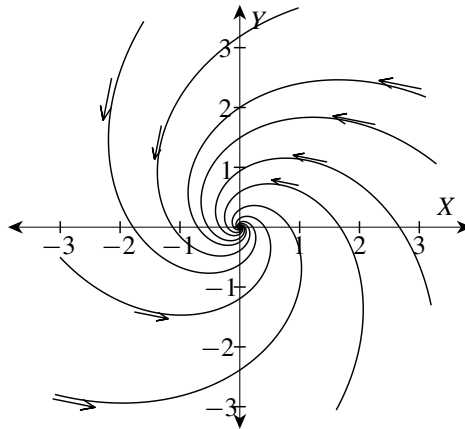
Figure 40.3: A phase portrait for \mathbf{x}' = \mathbf{A}\mathbf{x} for a case where \mathbf{A} has complex eigenvalues with negative real parts.
