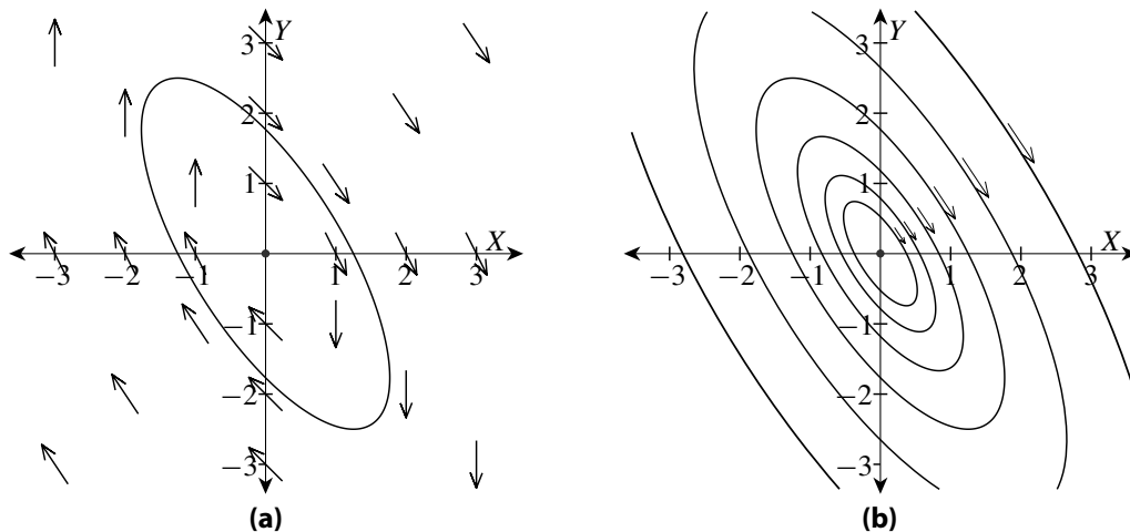
Figure 40.1: (a) A minimal direction field with one ‘matching’ elliptic trajectory, and (b) a phase portrait of the system in example 40.2.
