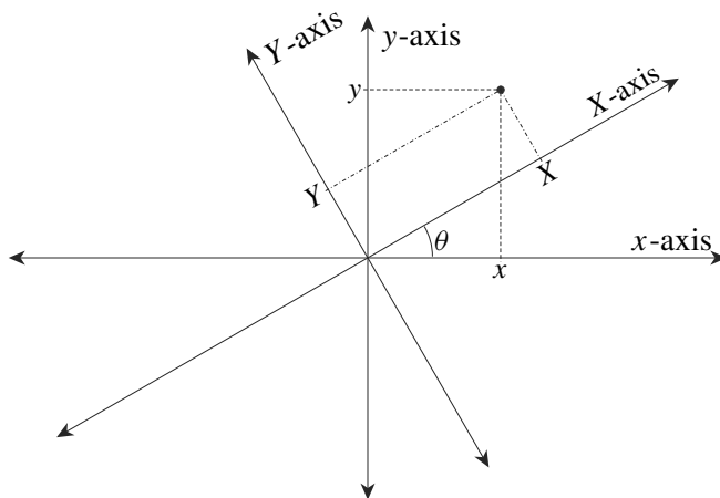
Figure 40.5: An XY -coordinate system obtained by rotating the xy -coordinate system by an angle \theta .
